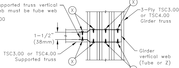
Section B-B If width of girder vertical web is: 2" (51mm) use clip TSHDC2.04 2-1/2" (64mm) use clip TSHDC2.54 3-1/2" (90mm) use clip TSHDC3.54
