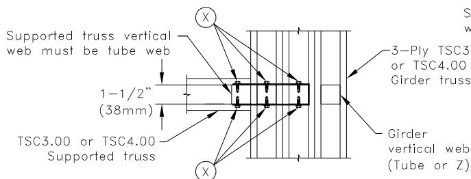
Section A-A If width of girder vertical web is: 1-1/2" (38mm) use clip TSCC664
